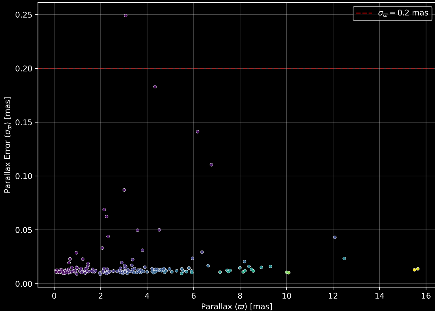
APOGEE DR17 Field: [070+53_MGA] Parallax Quality (n= 185)
