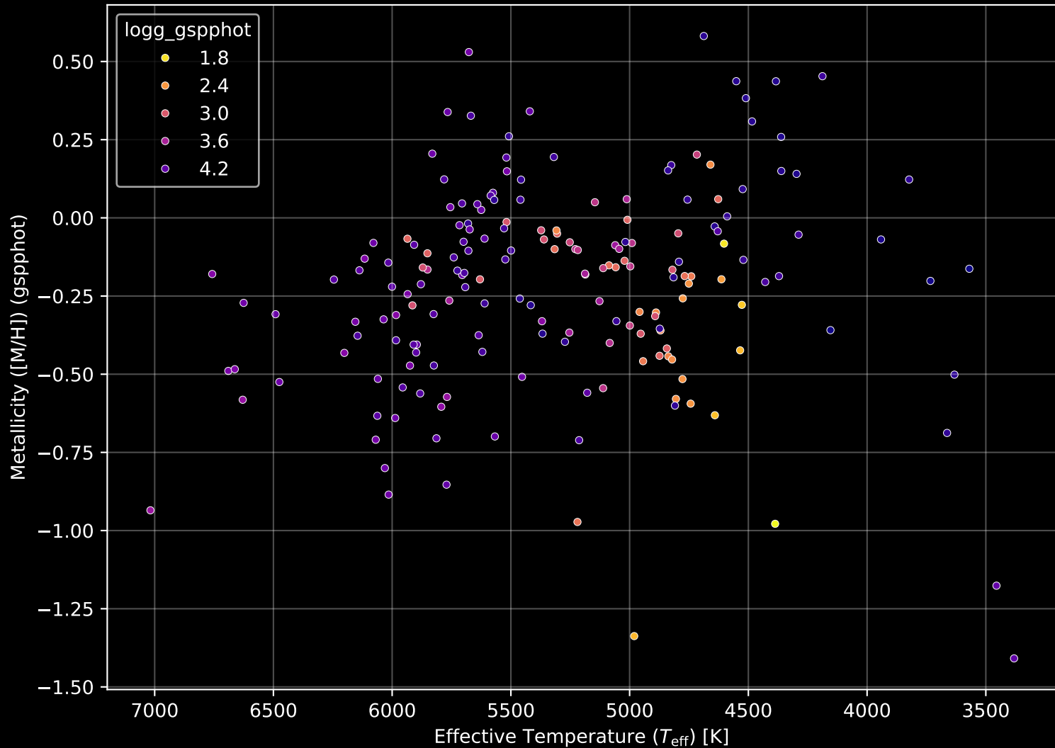
APOGEE DR17 Field: [070+53_MGA] Stellar Population Parameters (n= 185)
