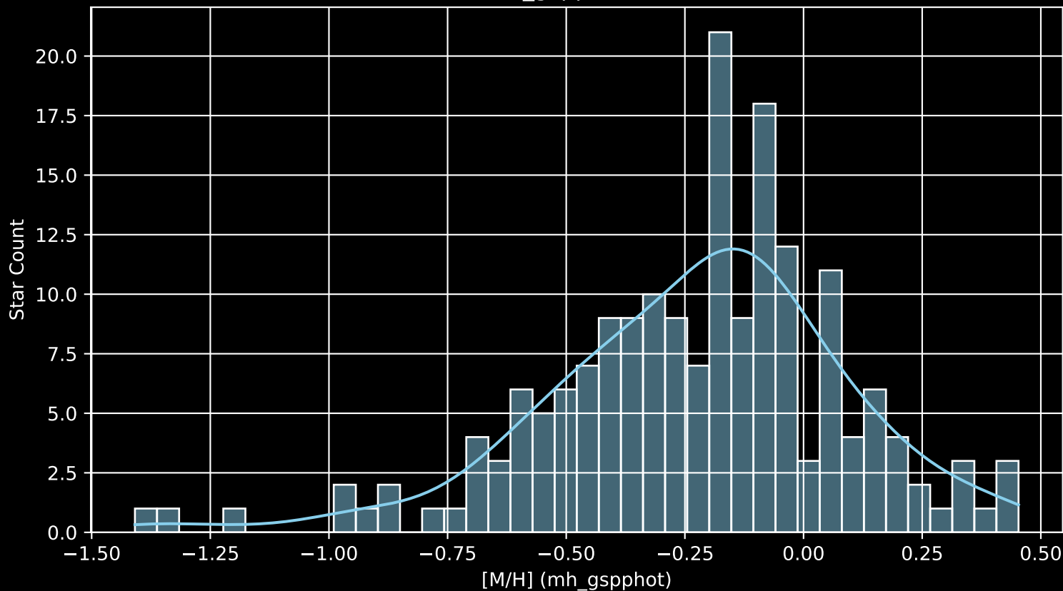
APOGEE DR17 Field: [070+53_MGA [M/H] (mh_gspphot) (n= 183)
