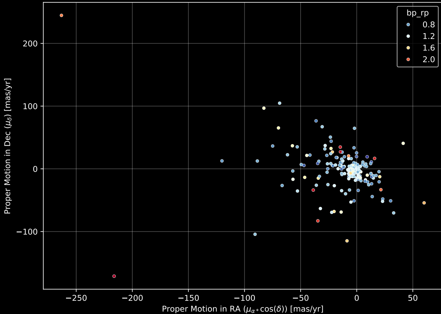
APOGEE DR17 Field: [070+53_MGA] Proper Motion Diagram (n= 185)
