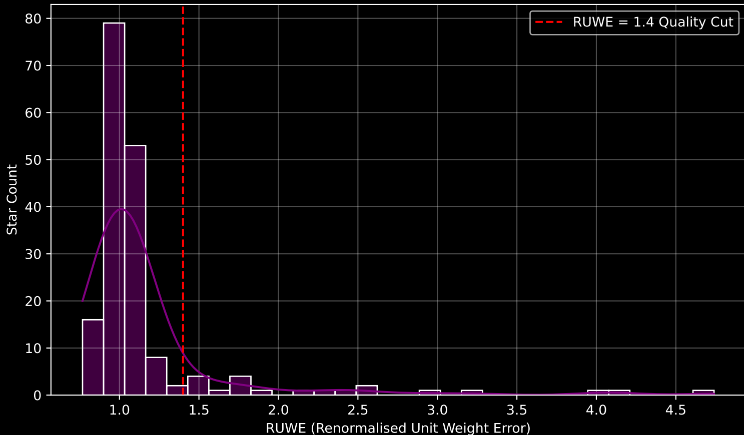
GAPOGEE DR17 Field [070+53_MGA] RUWE Distribution (n= 178)
