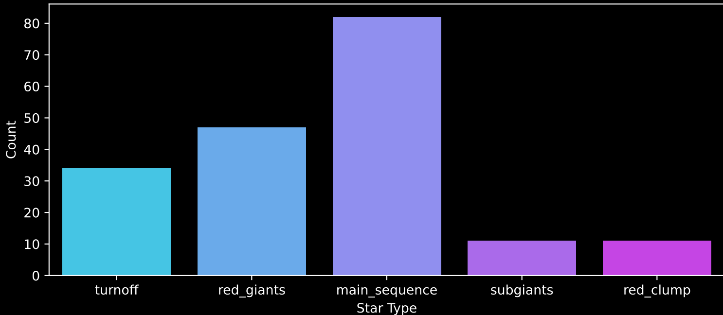
APOGEE DR17 Field: [070+53_MGA] Count plot of Star Type
